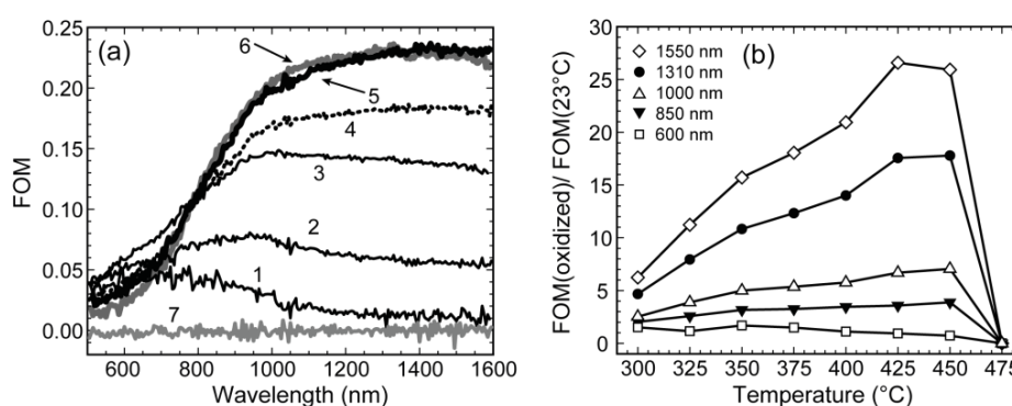
(a) Changes in \text{FOM} = \theta_F \sqrt{T} for the nanofilms: initial permalloy nanofilm (curve 1) and oxidized ones during annealing for one hour at the series of temperatures (curves 2-7 correspond to 300, 350, 400, 425, 450 and 475°C, respectively). (b) Normalized FOM for selected wavelengths versus the oxidation temperature.
