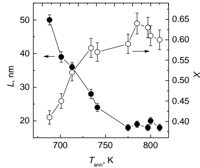
Fig. 2. Changes of average sizes of \alpha -Fe nanocrystals (●) and their volume fraction (○) vs. temperatures of annealing up to end nanocrystallization
