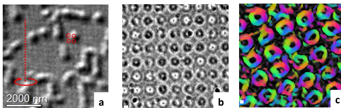
Fig. 1. LTEM images of a lattice of magnetic bubbles in a demagnetized state. The observed contrast corresponds to the distribution of magnetization for Neel (a) and Bloch (b) skyrmions; (c) reconstructed magnetization distributions from LTEM micrographs with differential phase contrast. It is observed from the skyrmion with both right and left helicity.
