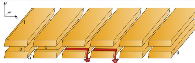
Fig. 1. Array of magnetic microwave guides
