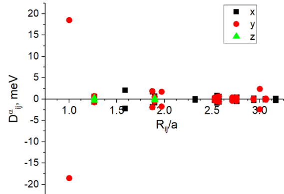
Fig.3. Components of Dzyaloshinskii-Moriya interaction vector between Tb atoms.
