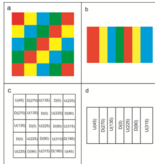
Fig.2 The regular stripe structures: linear (b,d) and checkerboard (a,c). R color – U( \theta = 45^\circ ) stripe, Y - D( \theta = 270^\circ ), B - U( \theta = 135^\circ ), G – D( \theta = 0^\circ ) in stripe group G(\varphi) .
