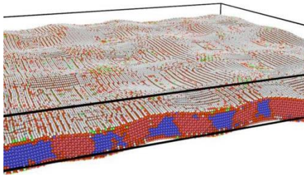
Fig. 1. Formation of the TiNi austenite phase simulated using the MD method within the LAMMPS package. The blue color denotes austenite (B2), the red color - martensite phase (B19).
