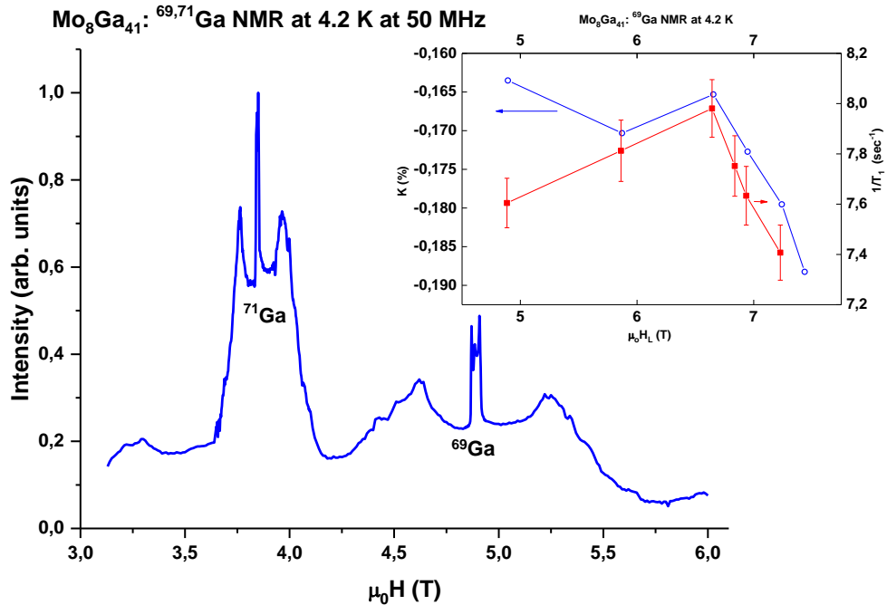
Fig. 1. \text{Mo}_8\text{Ga}_{41} field-sweep NMR spectrum at 50 \text{ MHz} and 4.2 \text{ K} . Inset: ^{69}\text{Ga} Knight shift (left) and spin-lattice relaxation rate (right) as a function of magnetic field.
