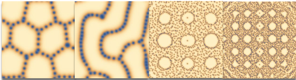
Fig. 1. Examples of the self-dual patterns of the superconducting condensate (yellow color corresponds to the bulk value of the condensate density, points represent vortices). One can see the bubble (islands) and stripe patterns in their complex interplay with the Nielsen-Olesen vortices.
