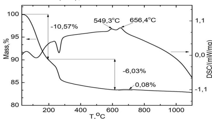
Fig.1. TG and DSC curves for PPT-Mn/Al (1:1)
