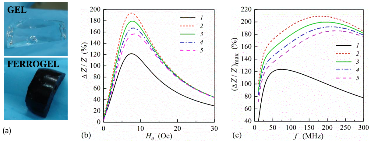
Fig. 1. General view of polyacrylamide gel and ferrogel filled with \text{Fe}_2\text{O}_3 nanoparticles (a), calculated MI ratio as a function of the external field at f=100 MHz (b) and frequency dependence of the maximum MI ratio (c). Curves 1, multilayer without gel; curves 2, H_p=0 ; curves 3, H_p=0.25 Oe; curves 4, H_p=0.5 Oe; curves 5, H_p=0.75 Oe.
