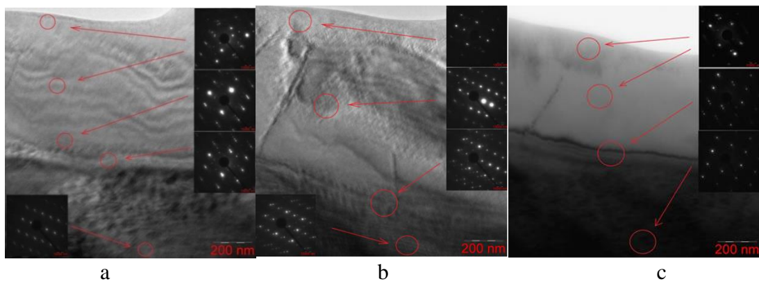
Fig. 1. Bright-field images and diffraction patterns of the selected regions of the \text{Ni}_{46}\text{Mn}_{41}\text{In}_{13} alloy at temperatures of 215 K (a), 208 K (b), 100 K (c).
