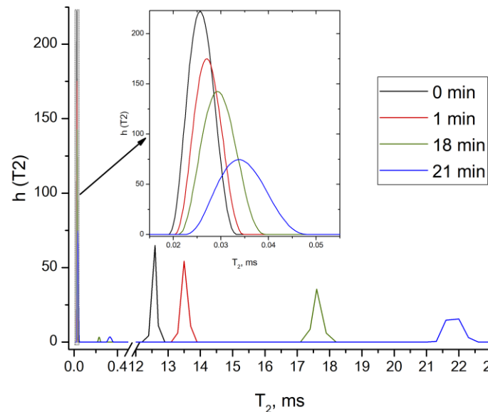
Fig.2. Transformation of relaxation time T_2 distribution for the magnetic fluid of c = 0.021 M in dc magnetic field
