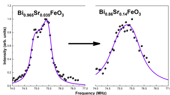
Figure 5. ^{57}\text{Fe} ZF-NMR spectra of \text{Bi}_{1-x}\text{Sr}_x\text{FeO}_3 for x = \{0.035; 0.14\} at 4.2 K This work was supported by grant 21-72-00112 from the Russian Science Foundation.
