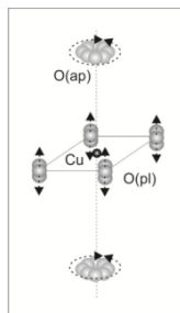
Fig.3 Dynamic picture for CuO 6 octahedra tunneling across U( \theta ) and D( \theta ) stripe positions. Tilting angle \varphi = \text{const} .
