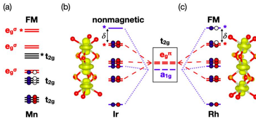
Figure 1: (a) Level diagram (with both t_{2g} and e_g^{\sigma} ) for Mn trimer (localized electrons) and (b), (c) scheme of t_{2g} energy levels (no e_g^{\sigma} ) for MO model and charge densities of the band above/at the Fermi level for (b) Ir and (c)
