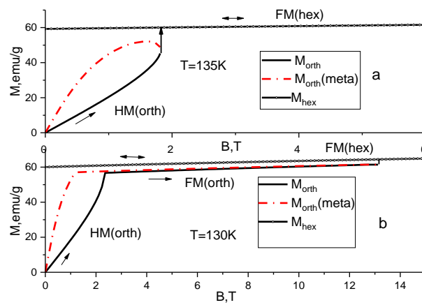
Fig.2 Isothermal field dependences of magnetization (model). a- irreversible ( \rightarrow ) magnetostructural \text{HM}(\text{orth}) \rightarrow \text{FM}(\text{hex}) ; b- reversible ( \leftrightarrow ) isostructural \text{HM}(\text{orth}) \leftrightarrow \text{FM}(\text{orth}) , irreversible ( \rightarrow ) magnetostructural transitions \text{FM}(\text{orth}) \rightarrow \text{FM}(\text{hex}) .
