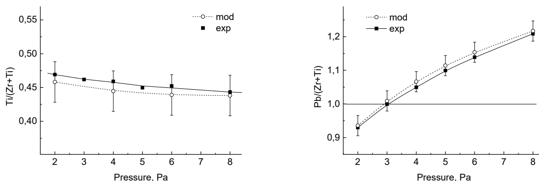
Fig. 1. Comparison of experimental and statistical modeling results for the elemental composition of \text{Ti}/(\text{Ti}+\text{Zr}) (left) \text{Pb}/(\text{Zr} + \text{Ti}) (right) in PZT thin films under gas pressure changing.
